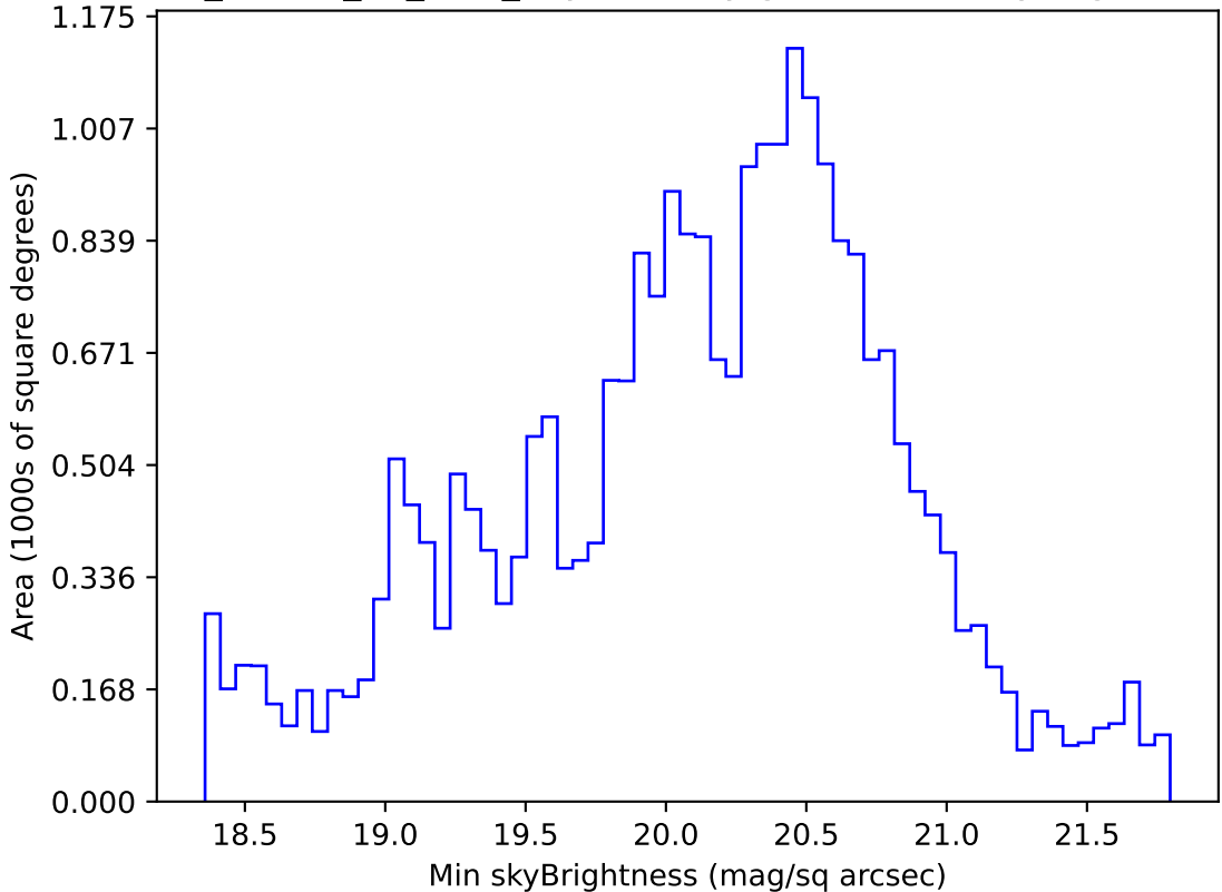
ddf_loaded_fl8_v3.4_10yrs All sky g band: Min skyBrightness
