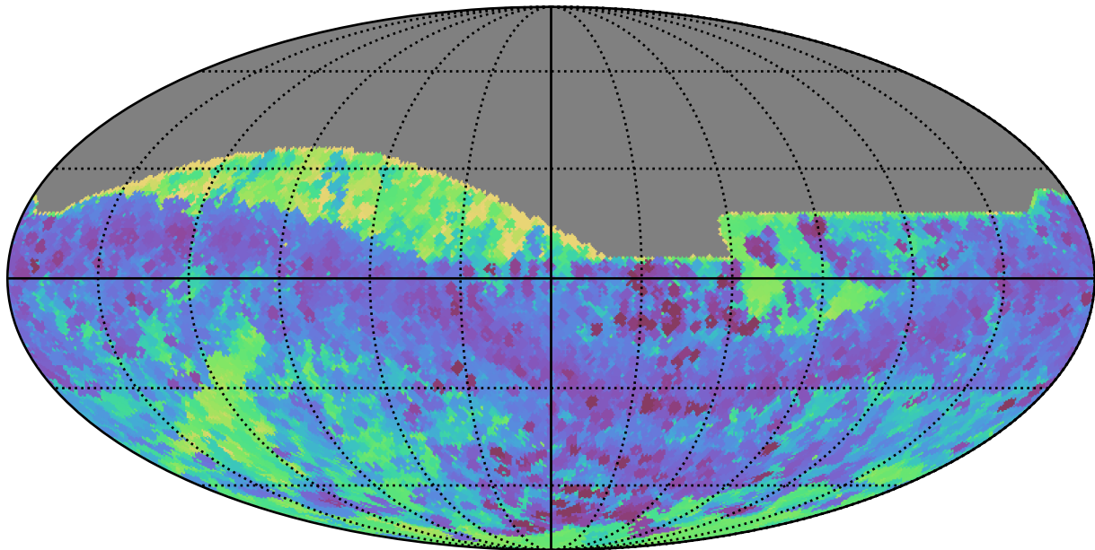
ddf_loaded_fl8_v3.4_10yrs All sky all bands: Min skyBrightness
