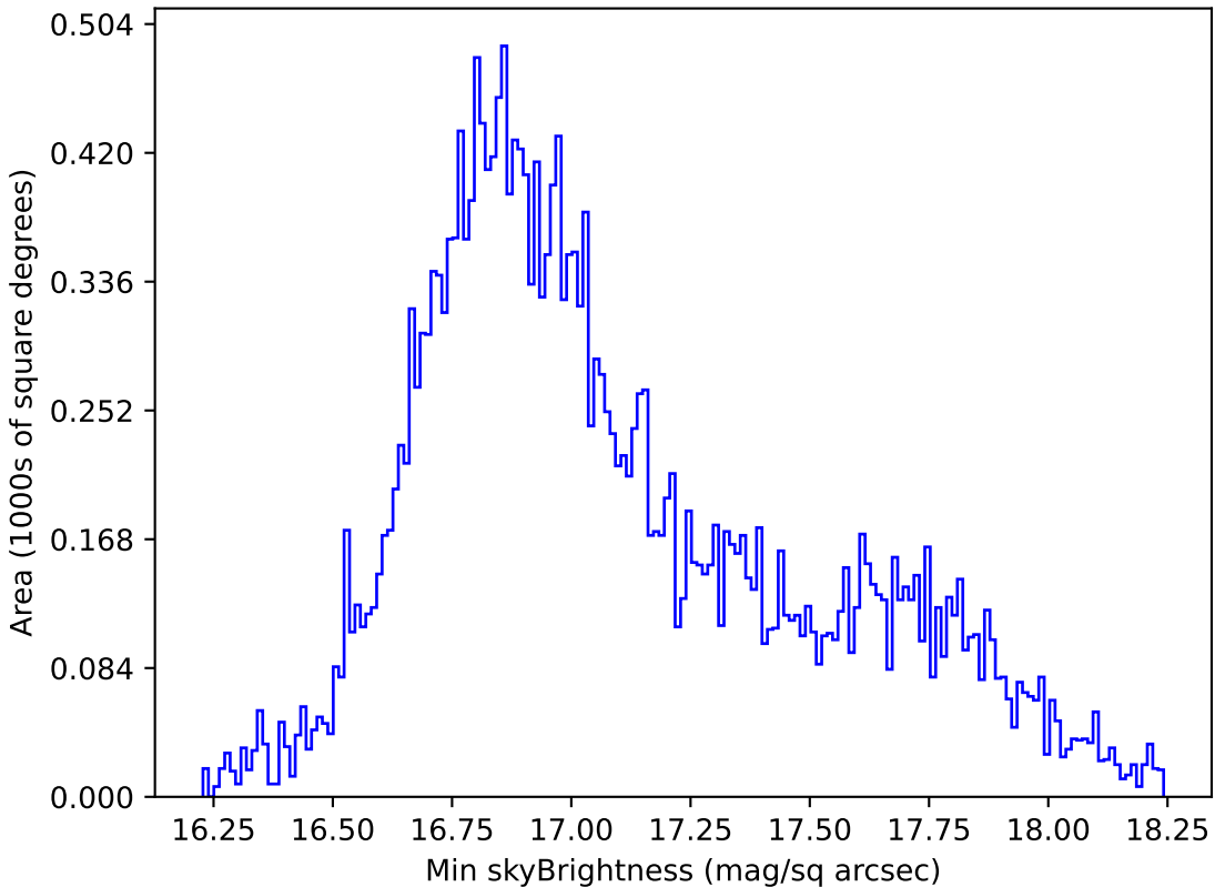
ddf_loaded_fl8_v3.4_10yrs All sky all bands: Min skyBrightness
