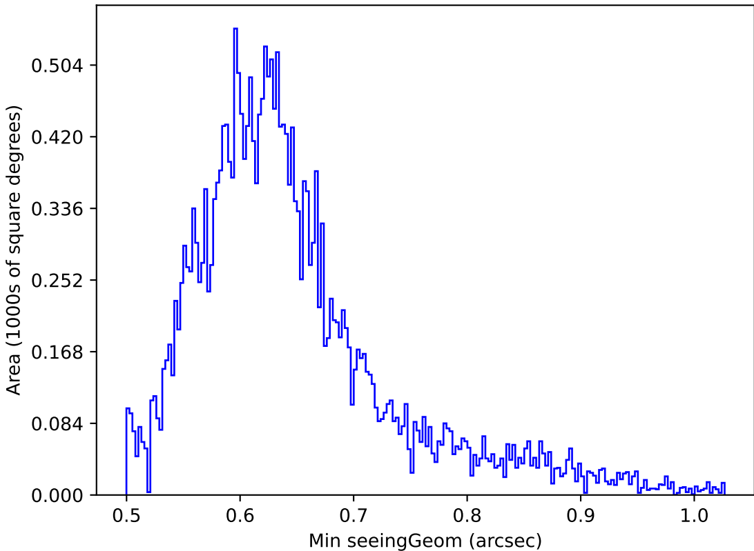
ddf_loaded_fl8_v3.4_10yrs Yr 1 z band: Min seeingGeom
