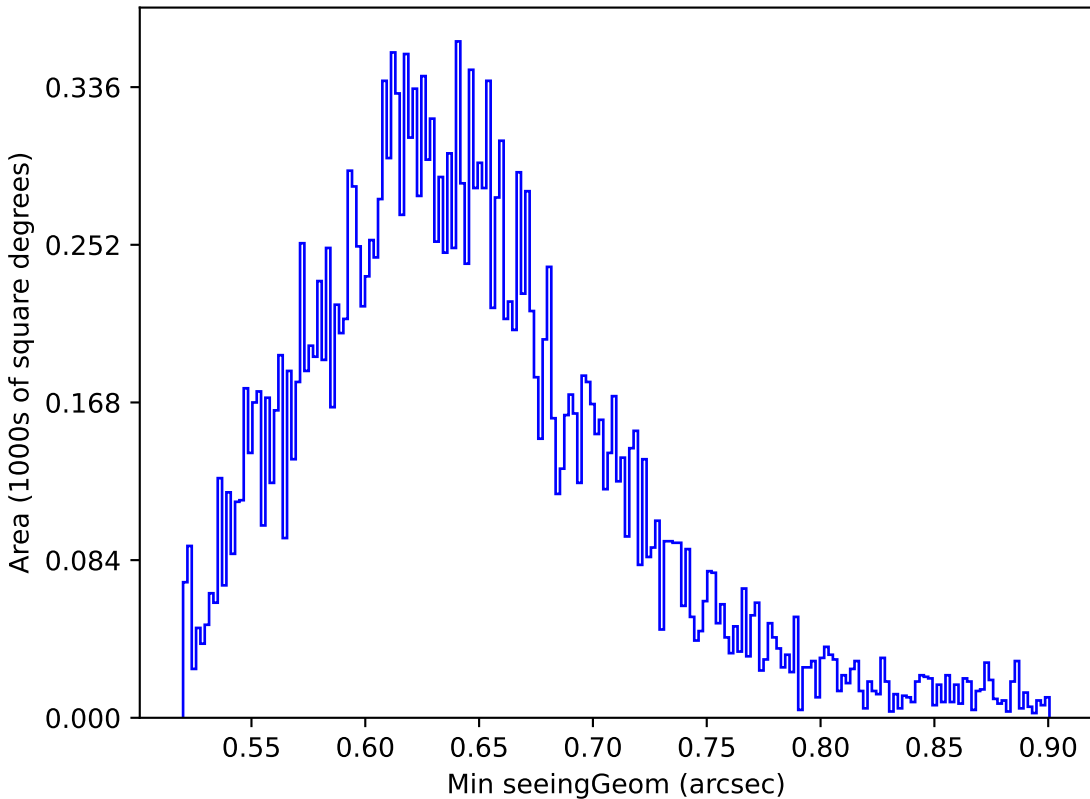
ddf_loaded_fl8_v3.4_10yrs Yr 1 y band: Min seeingGeom
