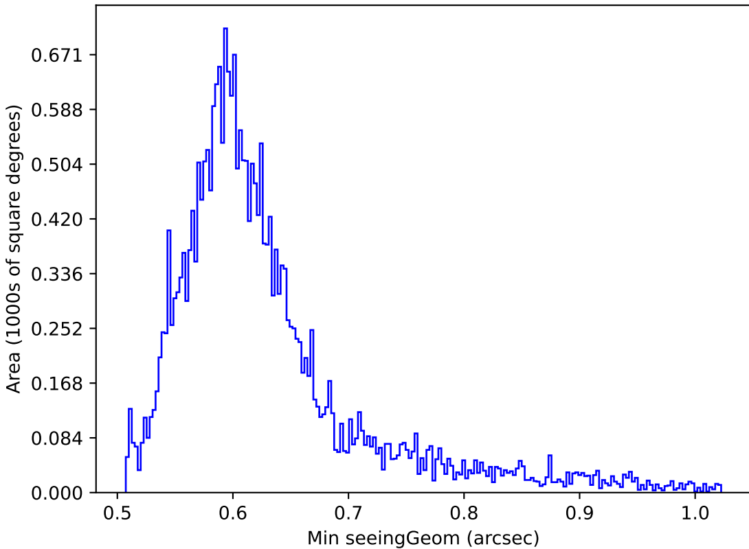
ddf_loaded_fl8_v3.4_10yrs Yr 1 i band: Min seeingGeom
