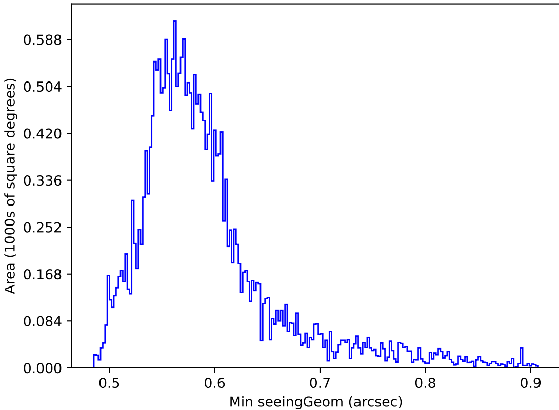
ddf_loaded_fl8_v3.4_10yrs Yr 1 all bands: Min seeingGeom
