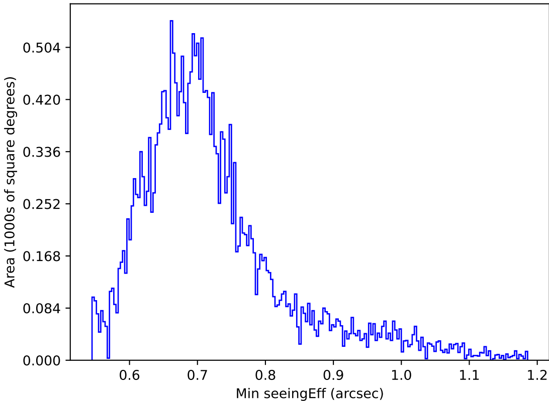
ddf_loaded_fl8_v3.4_10yrs Yr 1 z band: Min seeingEff
