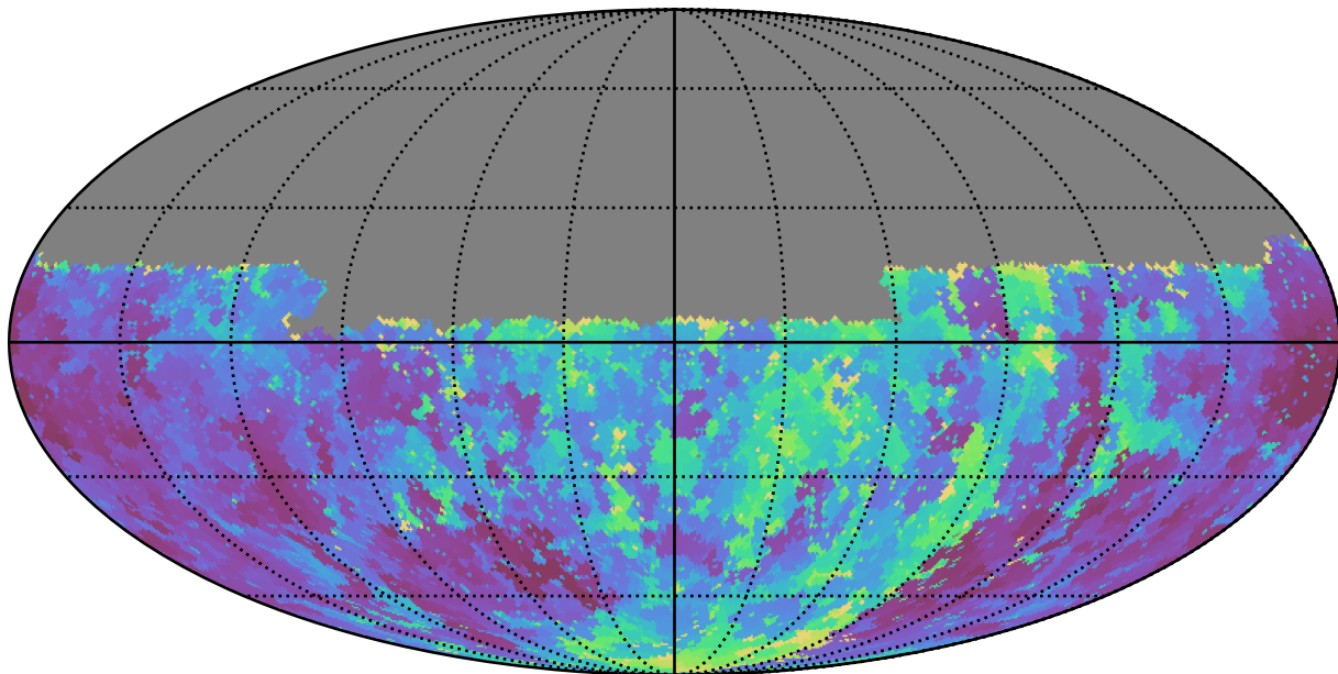
ddf_loaded_fl8_v3.4_10yrs Yr 1 u band: Min seeingEff
