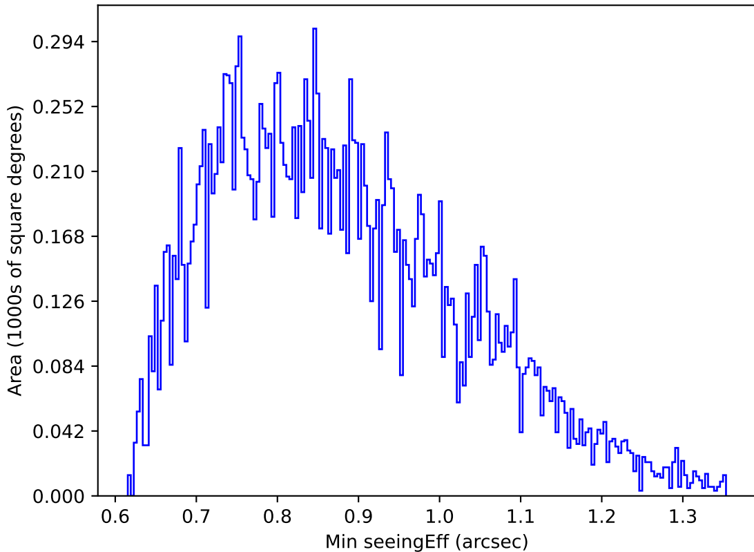
ddf_loaded_fl8_v3.4_10yrs Yr 1 u band: Min seeingEff
