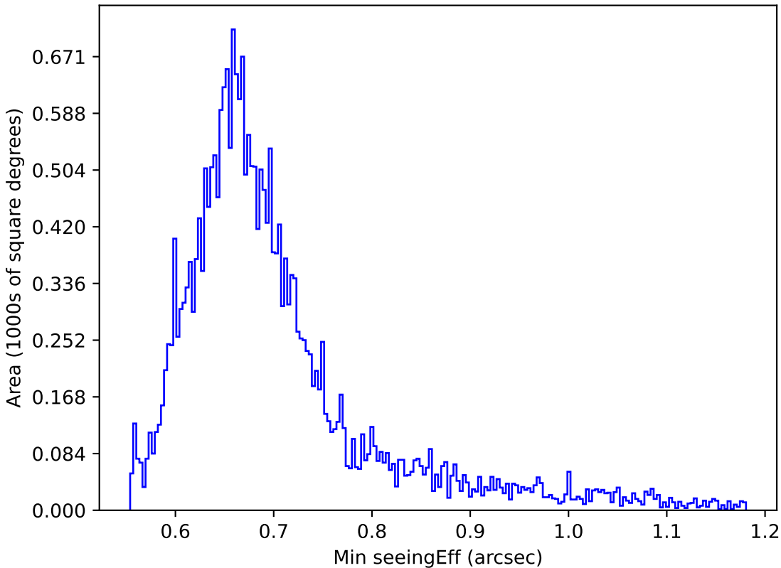
ddf_loaded_fl8_v3.4_10yrs Yr 1 i band: Min seeingEff
