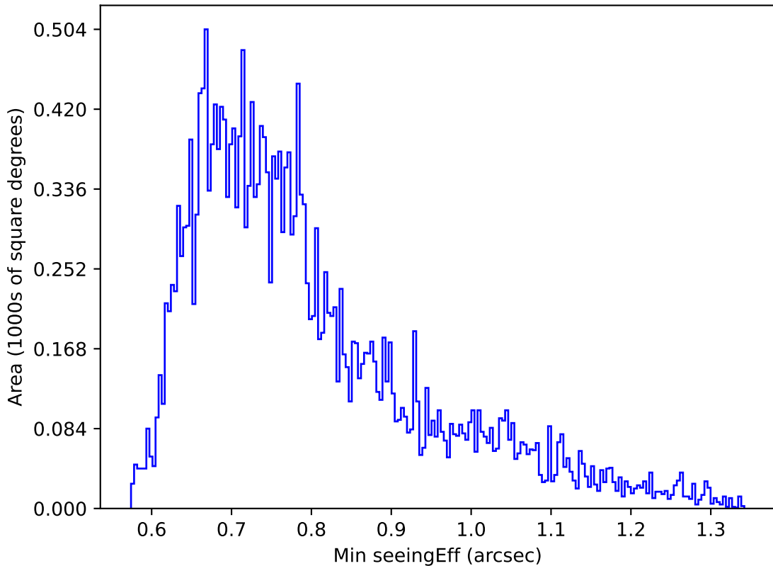
ddf_loaded_fl8_v3.4_10yrs Yr 1 g band: Min seeingEff
