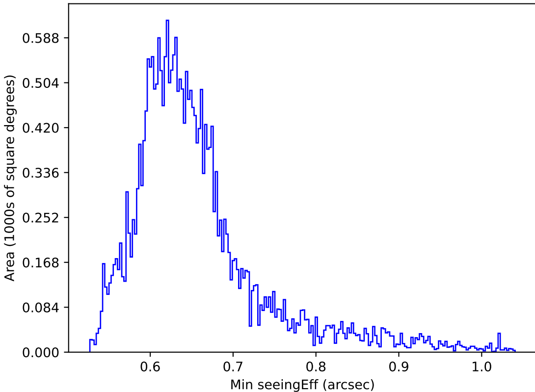
ddf_loaded_fl8_v3.4_10yrs Yr 1 all bands: Min seeingEff
