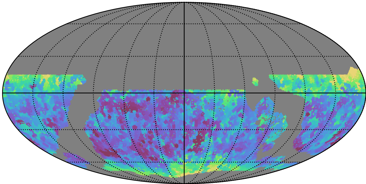
ddf_loaded_fl8_v3.4_10yrs WFD y band: Min seeingEff
