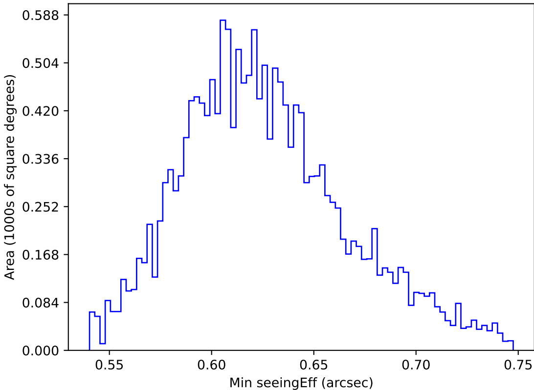
ddf_loaded_fl8_v3.4_10yrs WFD y band: Min seeingEff
