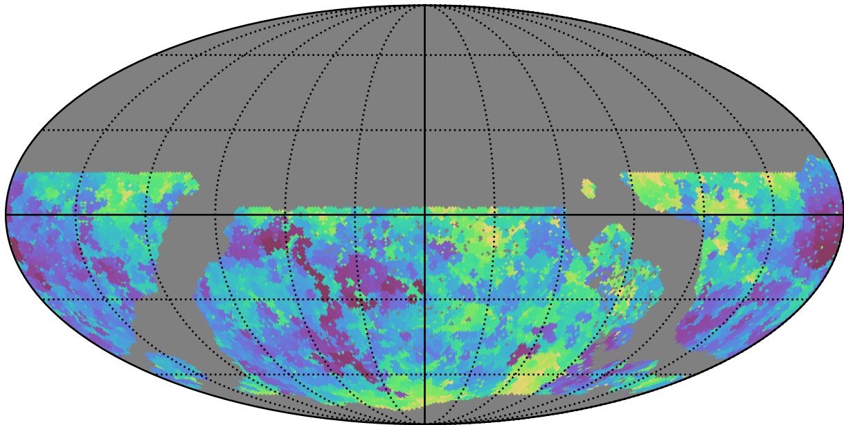
ddf_loaded_fl8_v3.4_10yrs WFD u band: Min seeingEff
