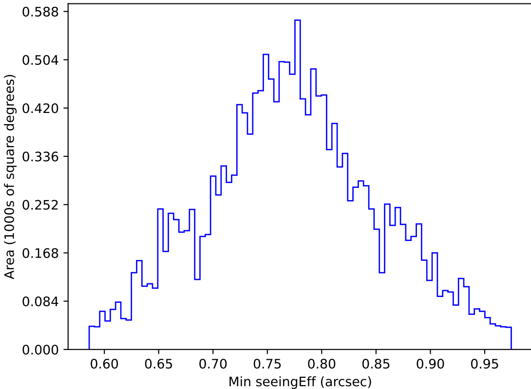
ddf_loaded_fl8_v3.4_10yrs WFD u band: Min seeingEff
