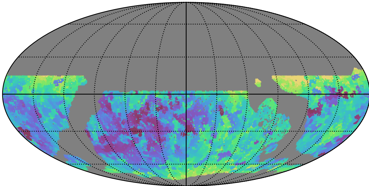
ddf_loaded_fl8_v3.4_10yrs WFD r band: Min seeingEff
