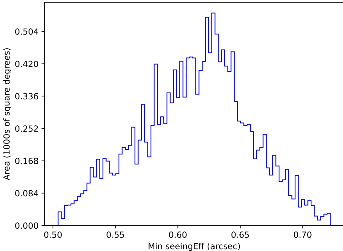
ddf_loaded_fl8_v3.4_10yrs WFD r band: Min seeingEff
