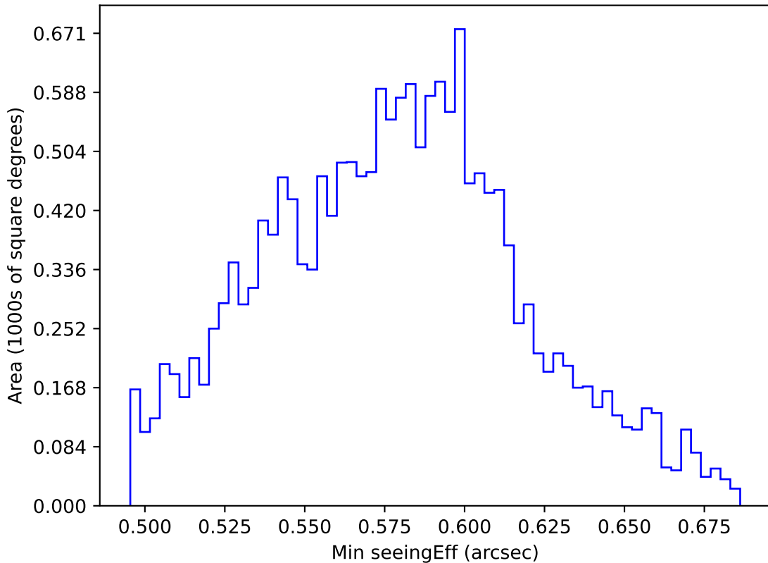
ddf_loaded_fl8_v3.4_10yrs WFD all bands: Min seeingEff
