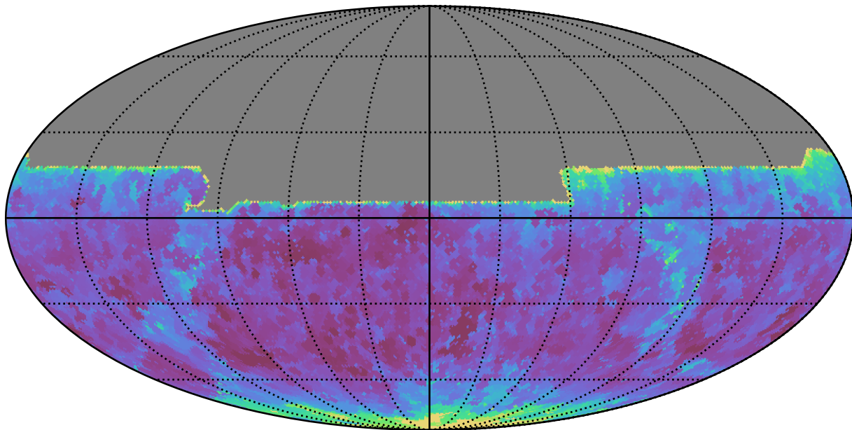
ddf_loaded_fl8_v3.4_10yrs All sky y band: Min seeingEff
