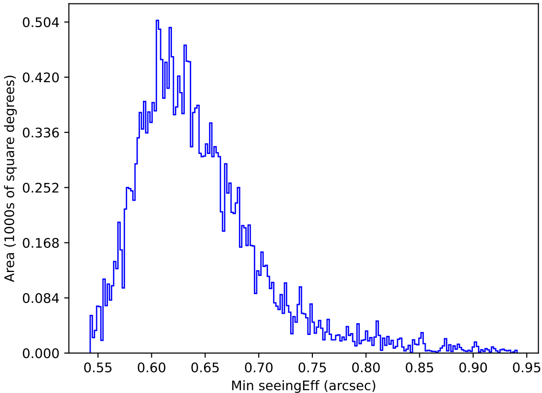
ddf_loaded_fl8_v3.4_10yrs All sky y band: Min seeingEff
