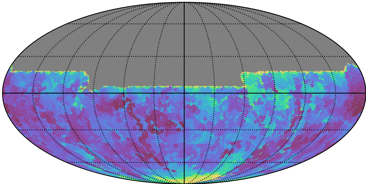
ddf_loaded_fl8_v3.4_10yrs All sky u band: Min seeingEff
