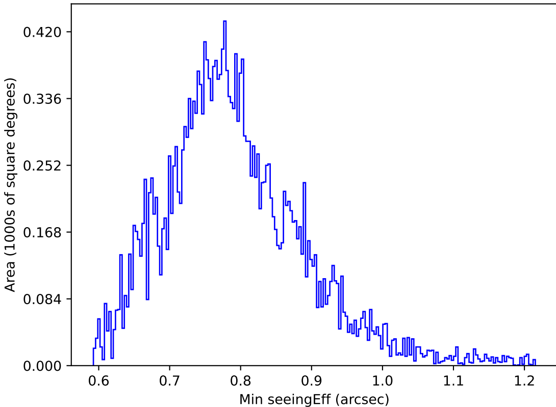
ddf_loaded_fl8_v3.4_10yrs All sky u band: Min seeingEff
