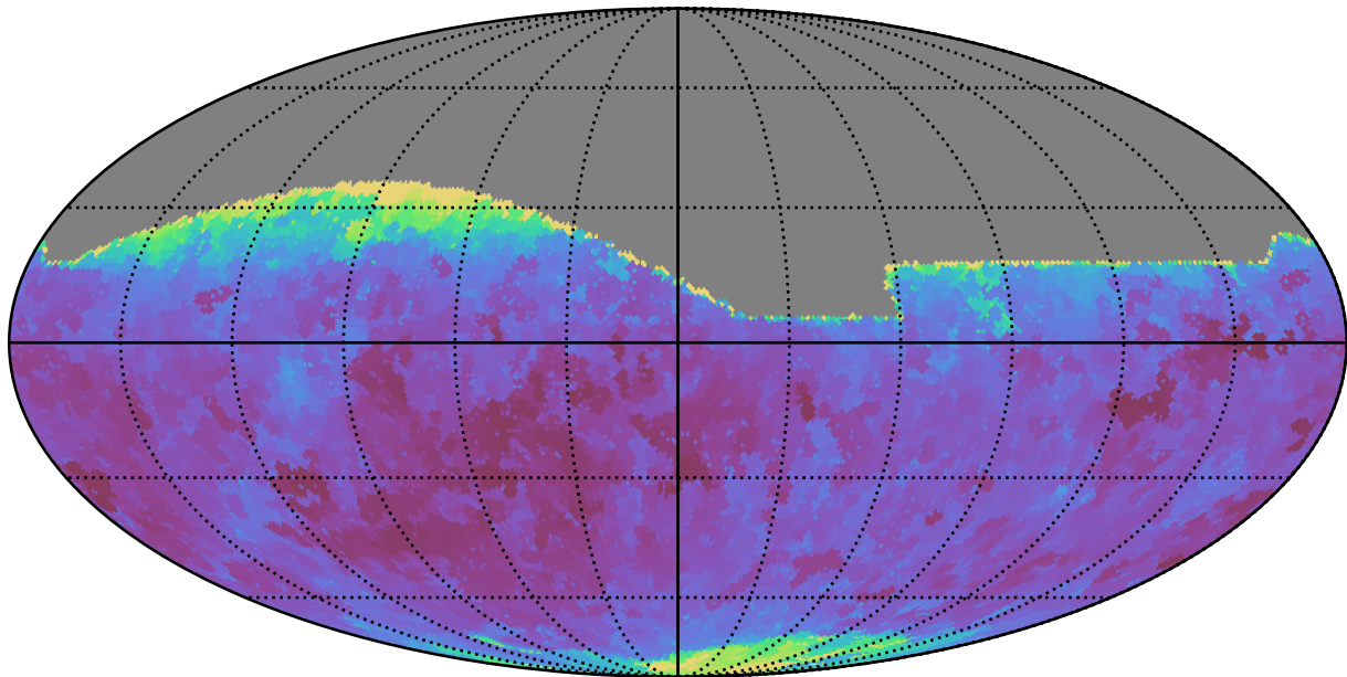
ddf_loaded_fl8_v3.4_10yrs All sky r band: Min seeingEff
