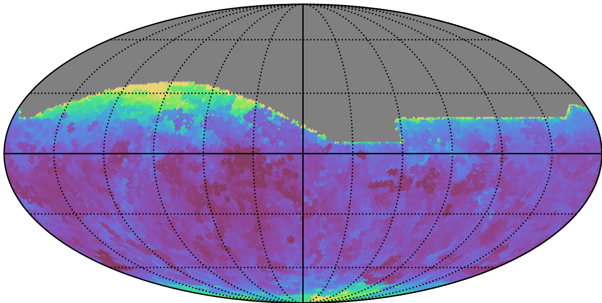
ddf_loaded_fl8_v3.4_10yrs All sky i band: Min seeingEff
