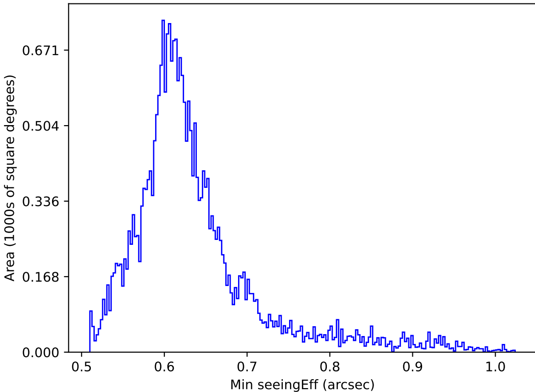
ddf_loaded_fl8_v3.4_10yrs All sky i band: Min seeingEff
