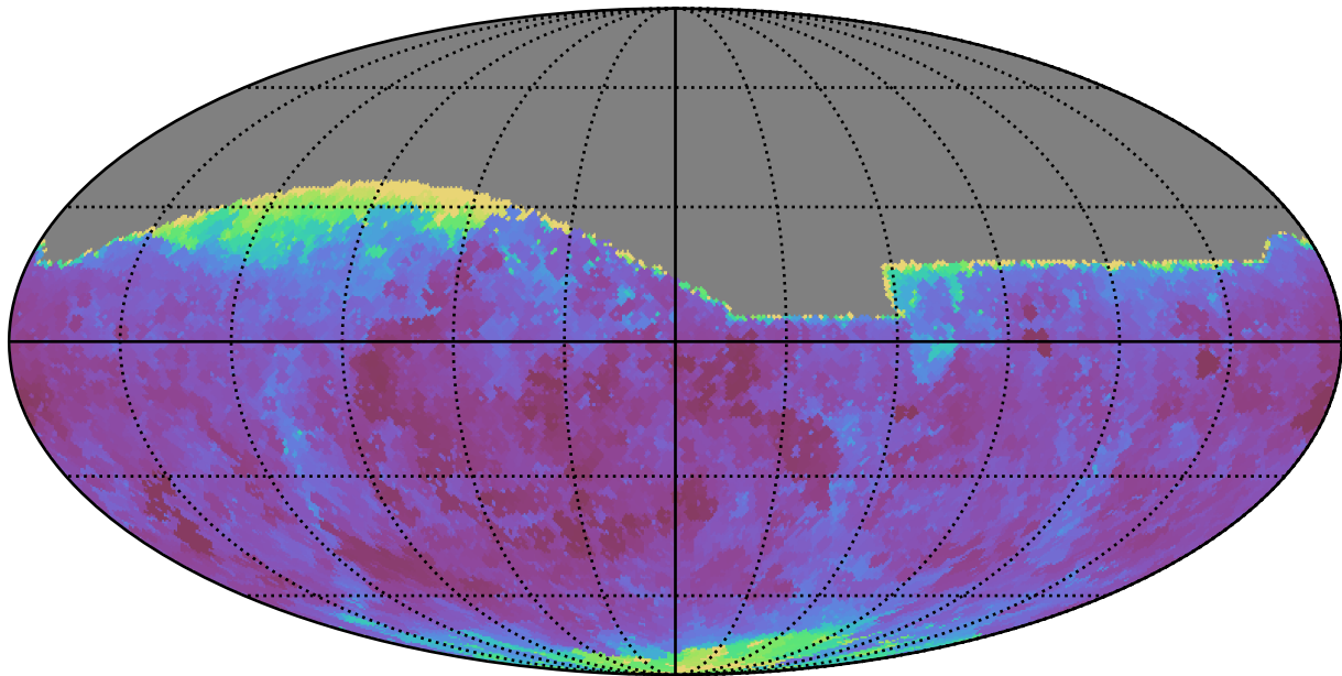
ddf_loaded_fl8_v3.4_10yrs All sky g band: Min seeingEff
