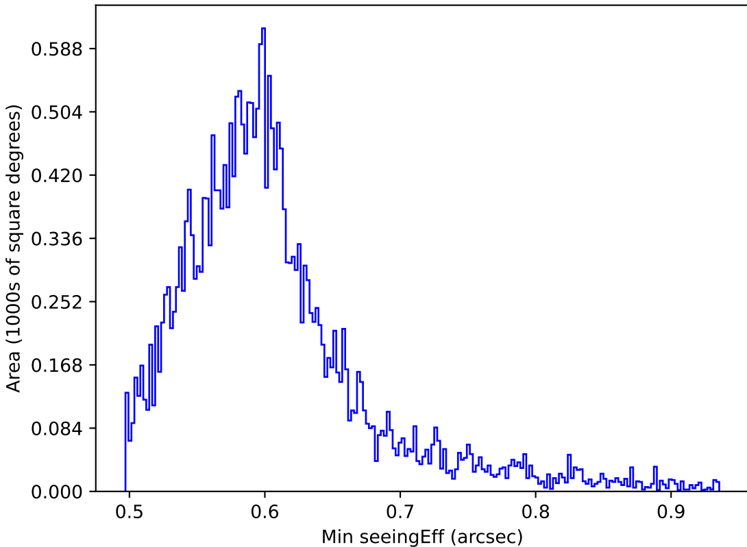
ddf_loaded_fl8_v3.4_10yrs All sky all bands: Min seeingEff
