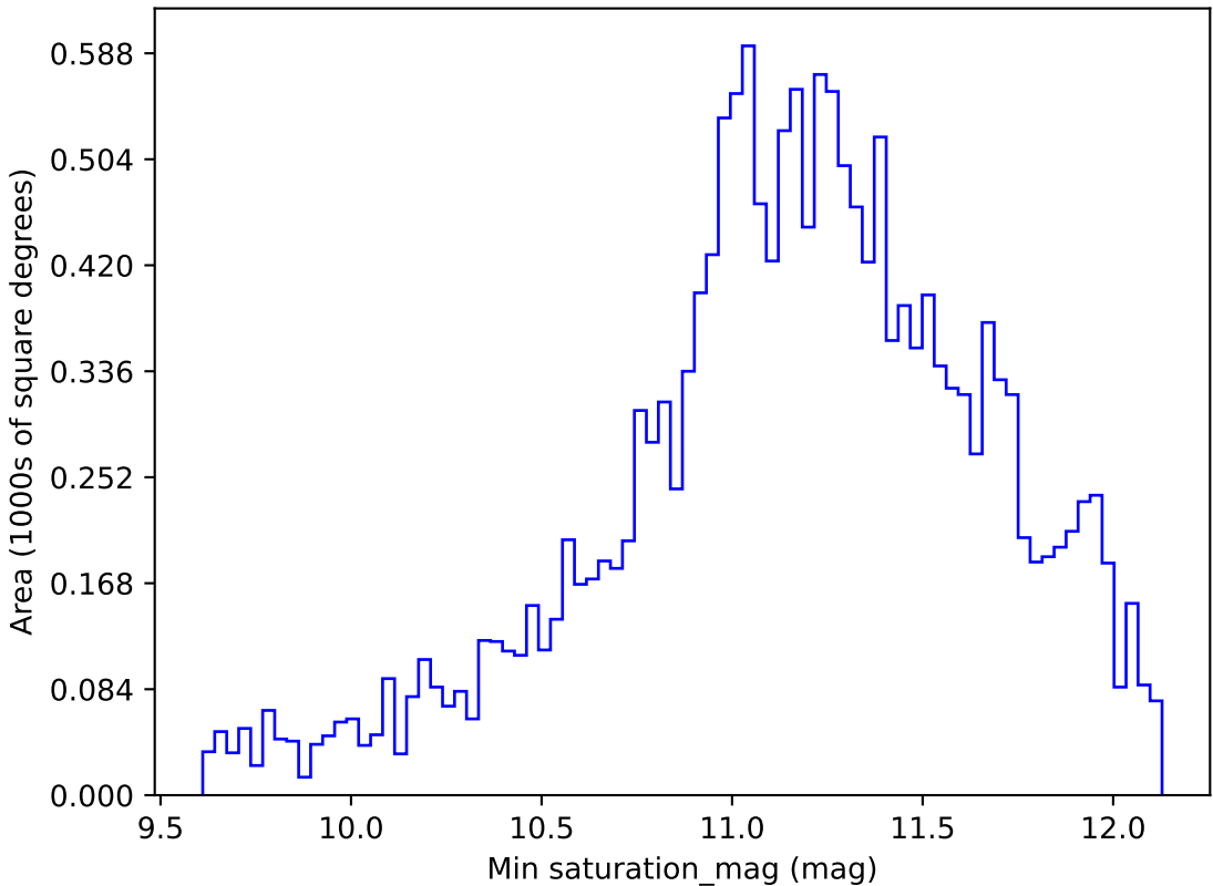
ddf_loaded_fl8_v3.4_10yrs WFD y band: Min saturation_mag
