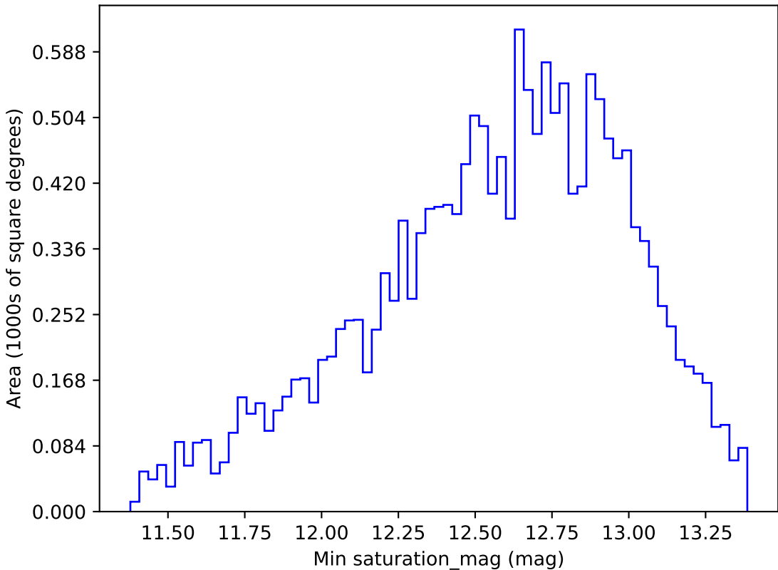
ddf_loaded_fl8_v3.4_10yrs WFD r band: Min saturation_mag
