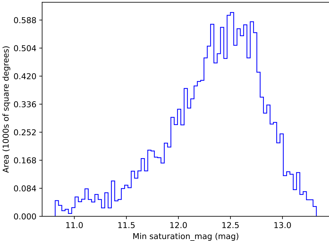
ddf_loaded_fl8_v3.4_10yrs WFD i band: Min saturation_mag
