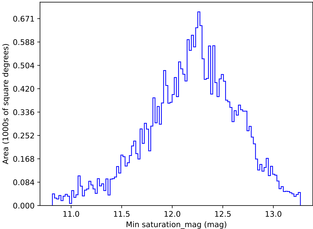
ddf_loaded_fl8_v3.4_10yrs All sky z band: Min saturation_mag
