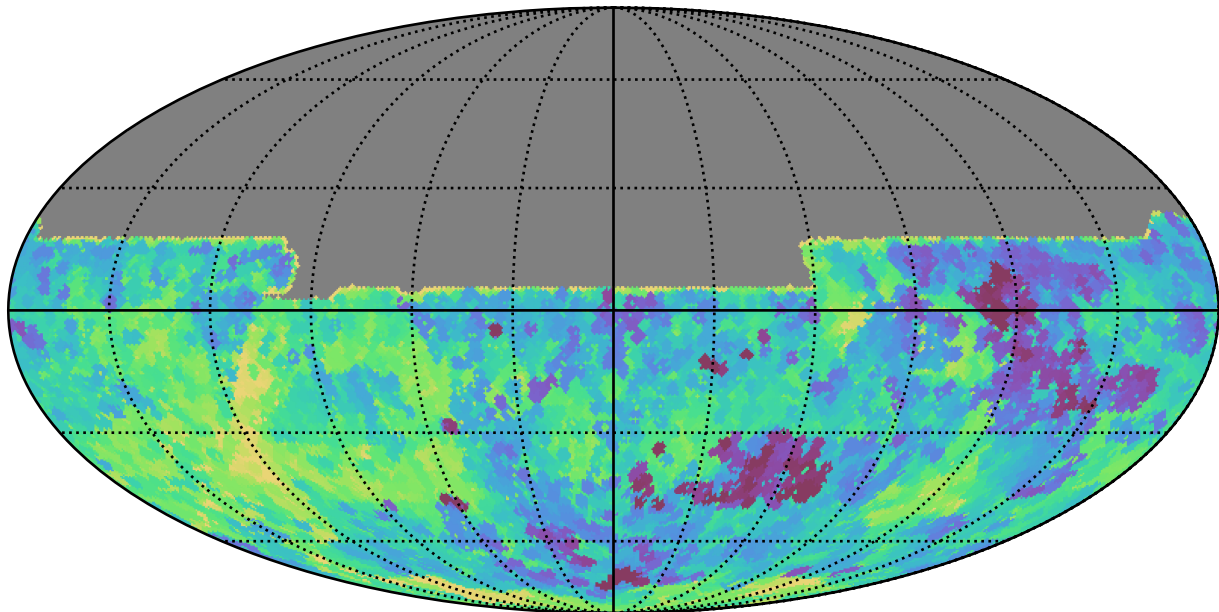
ddf_loaded_fl8_v3.4_10yrs All sky y band: Min saturation_mag
