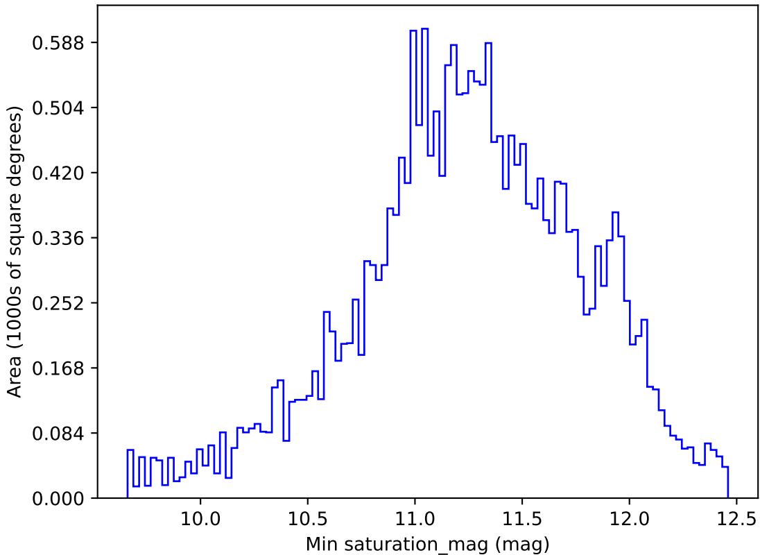
ddf_loaded_fl8_v3.4_10yrs All sky y band: Min saturation_mag
