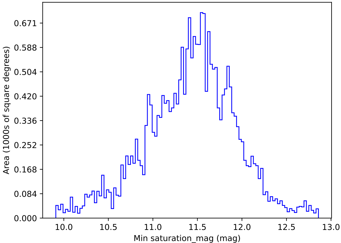
ddf_loaded_fl8_v3.4_10yrs All sky u band: Min saturation_mag
