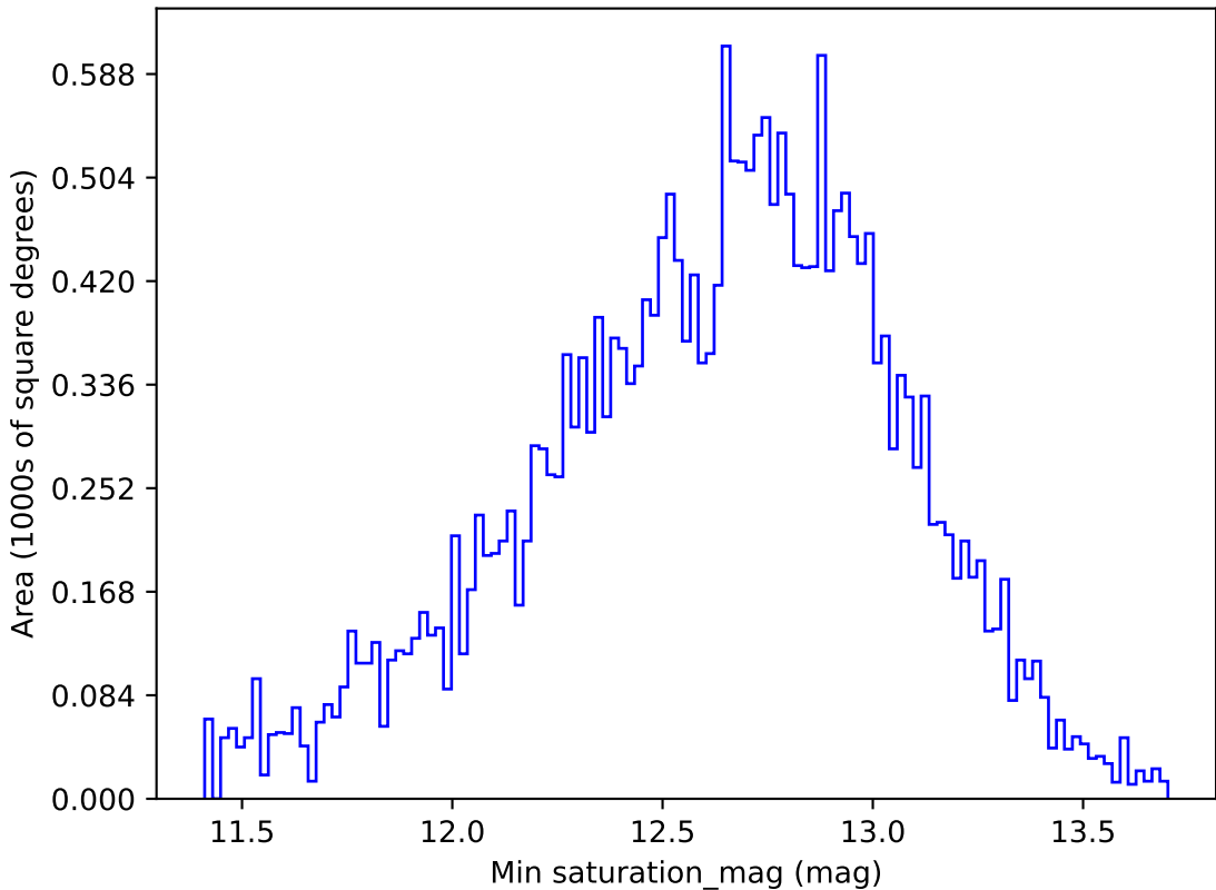
ddf_loaded_fl8_v3.4_10yrs All sky r band: Min saturation_mag
