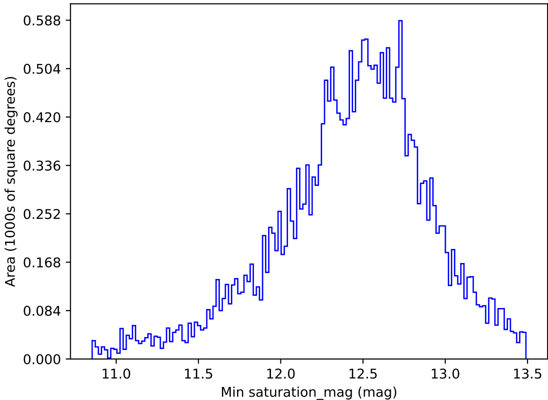
ddf_loaded_fl8_v3.4_10yrs All sky i band: Min saturation_mag
