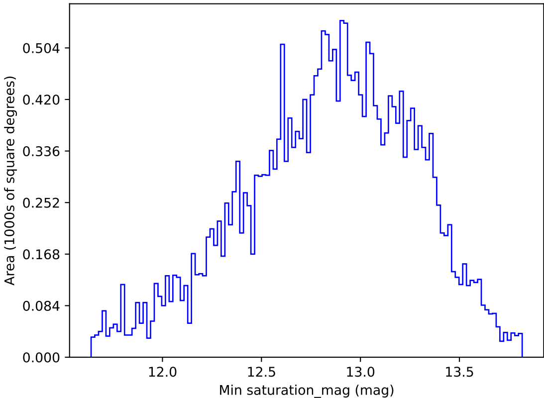
ddf_loaded_fl8_v3.4_10yrs All sky g band: Min saturation_mag
