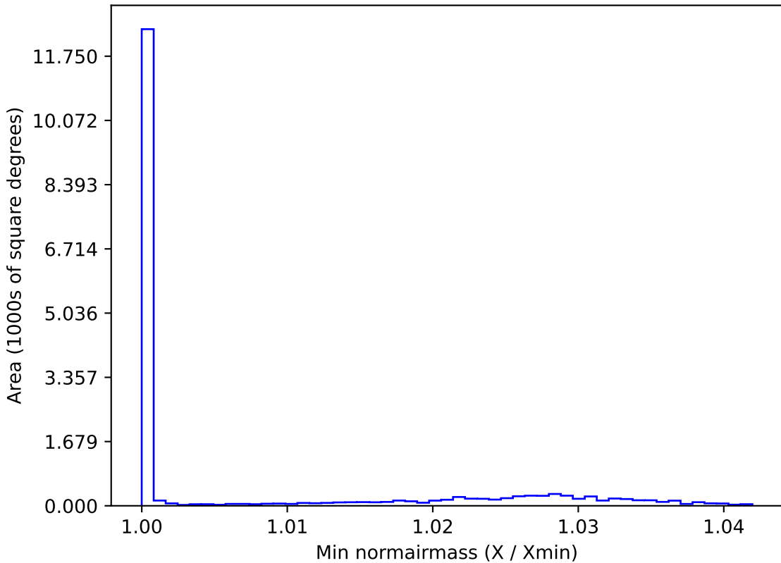
ddf_loaded_fl8_v3.4_10yrs WFD y band: Min normairmass
