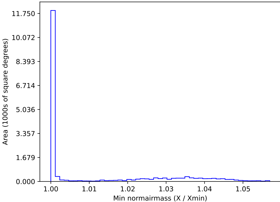
ddf_loaded_fl8_v3.4_10yrs WFD u band: Min normairmass
