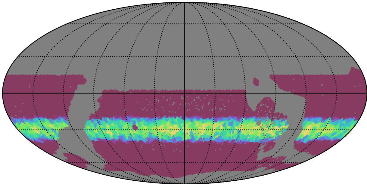
ddf_loaded_fl8_v3.4_10yrs WFD r band: Min normairmass
