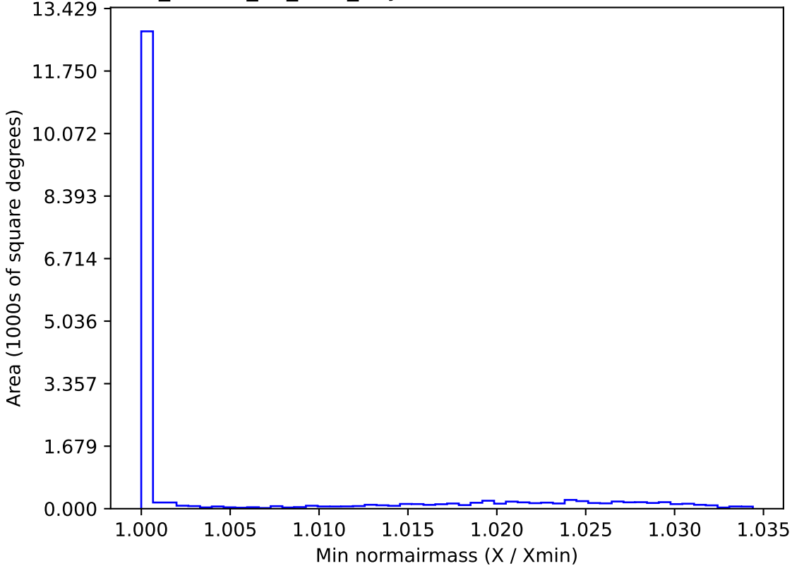
ddf_loaded_fl8_v3.4_10yrs WFD r band: Min normairmass
