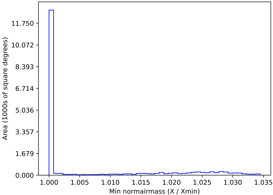
ddf_loaded_fl8_v3.4_10yrs WFD i band: Min normairmass
