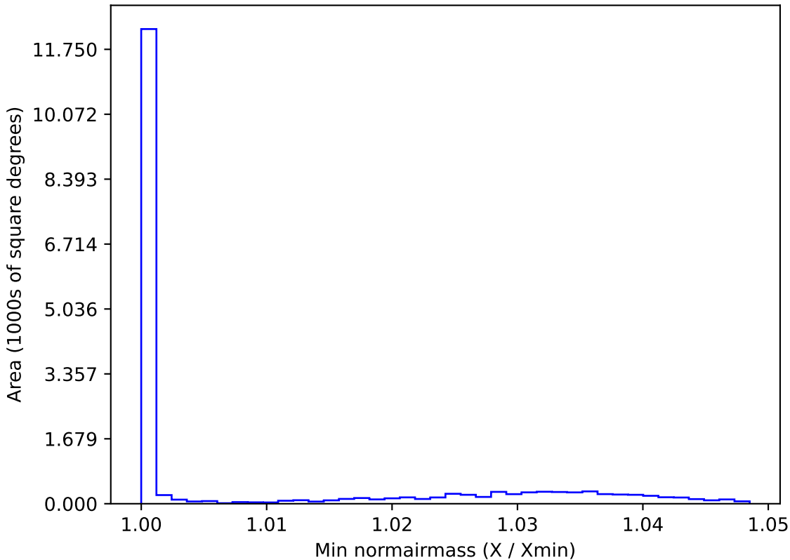
ddf_loaded_fl8_v3.4_10yrs WFD g band: Min normairmass
