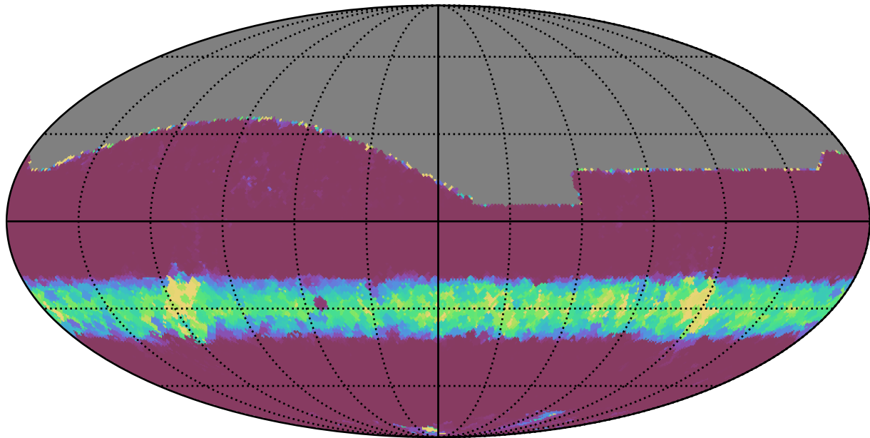
ddf_loaded_fl8_v3.4_10yrs All sky z band: Min normairmass
