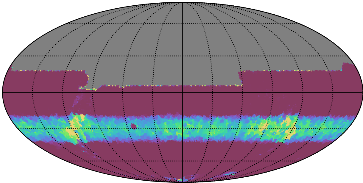
ddf_loaded_fl8_v3.4_10yrs All sky y band: Min normairmass
