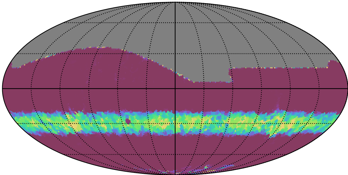
ddf_loaded_fl8_v3.4_10yrs All sky r band: Min normairmass
