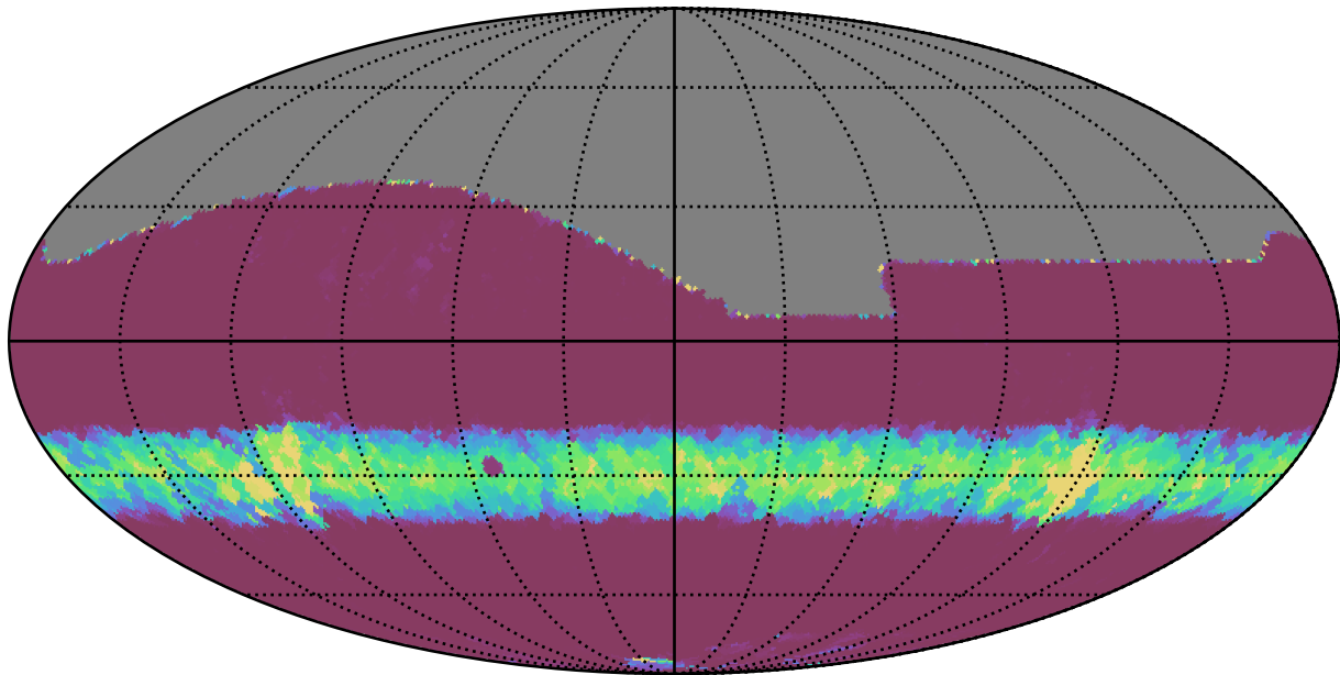
ddf_loaded_fl8_v3.4_10yrs All sky i band: Min normairmass
