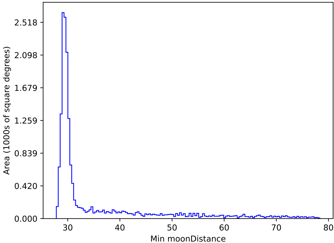
ddf_loaded_fl8_v3.4_10yrs WFD y band: Min moonDistance
